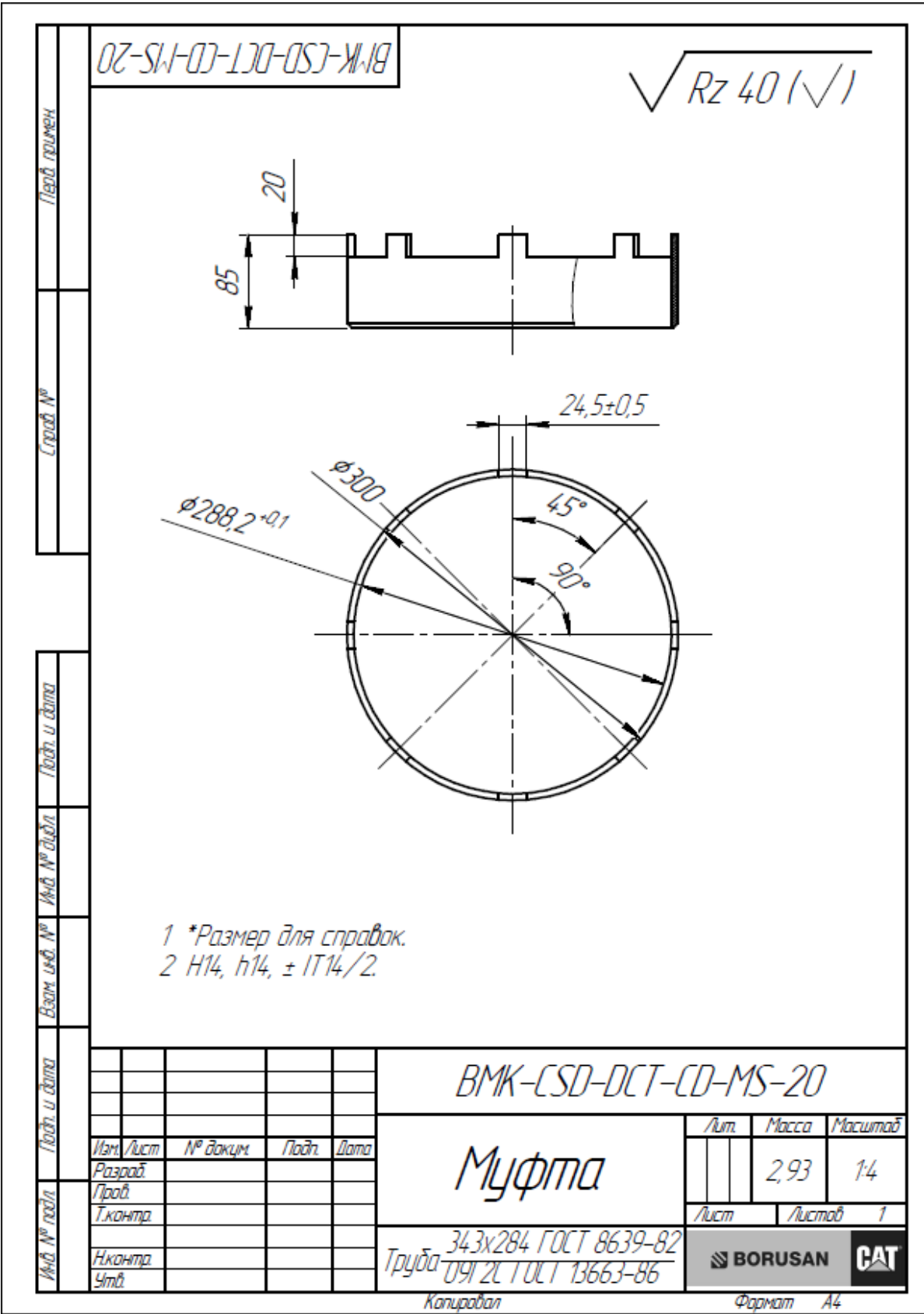
Drawing 3 coupling
