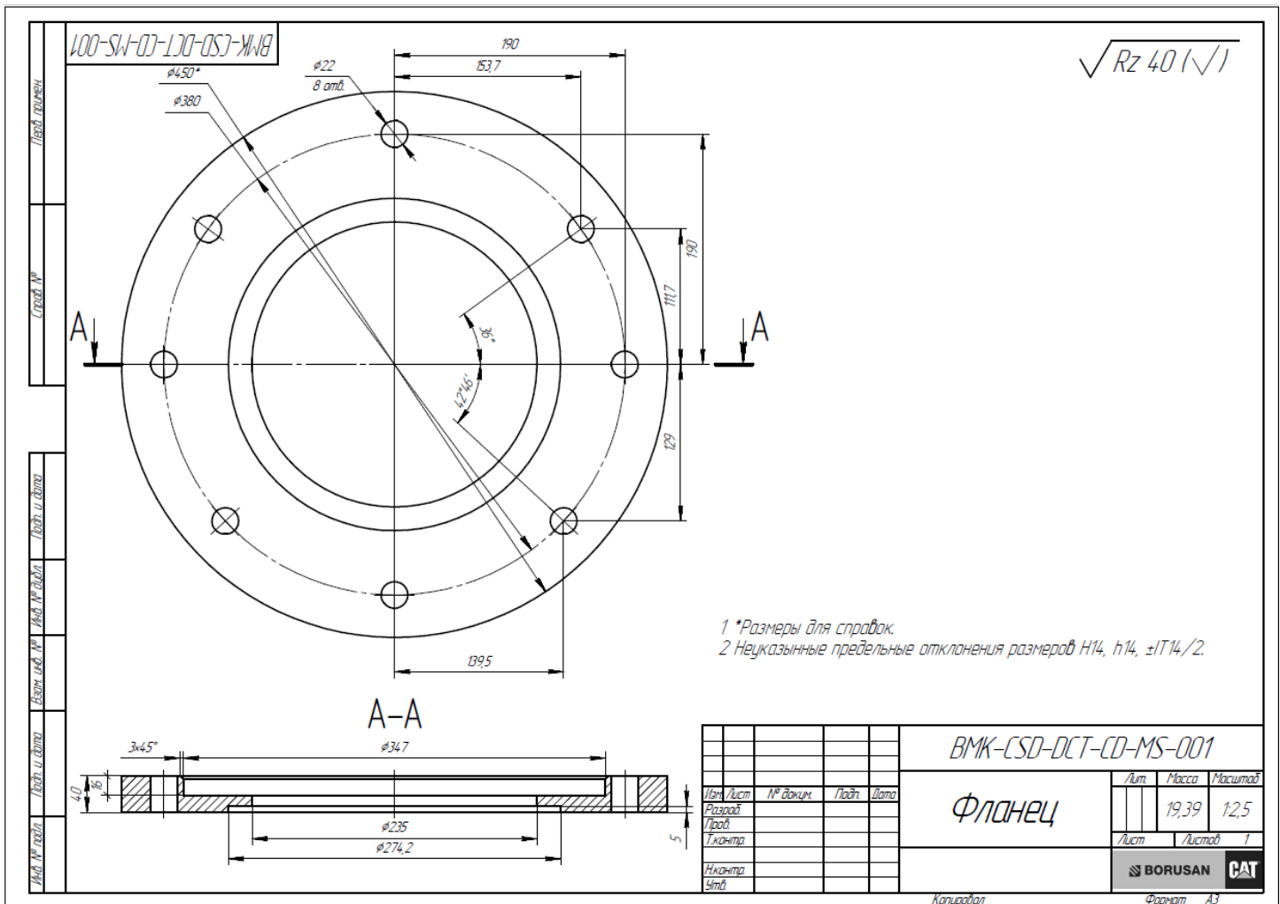
Drawing 9 flange
