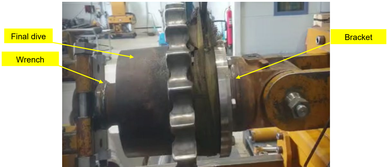
Fig. 3 tool for assembly, disassembly of the onboard final drive
