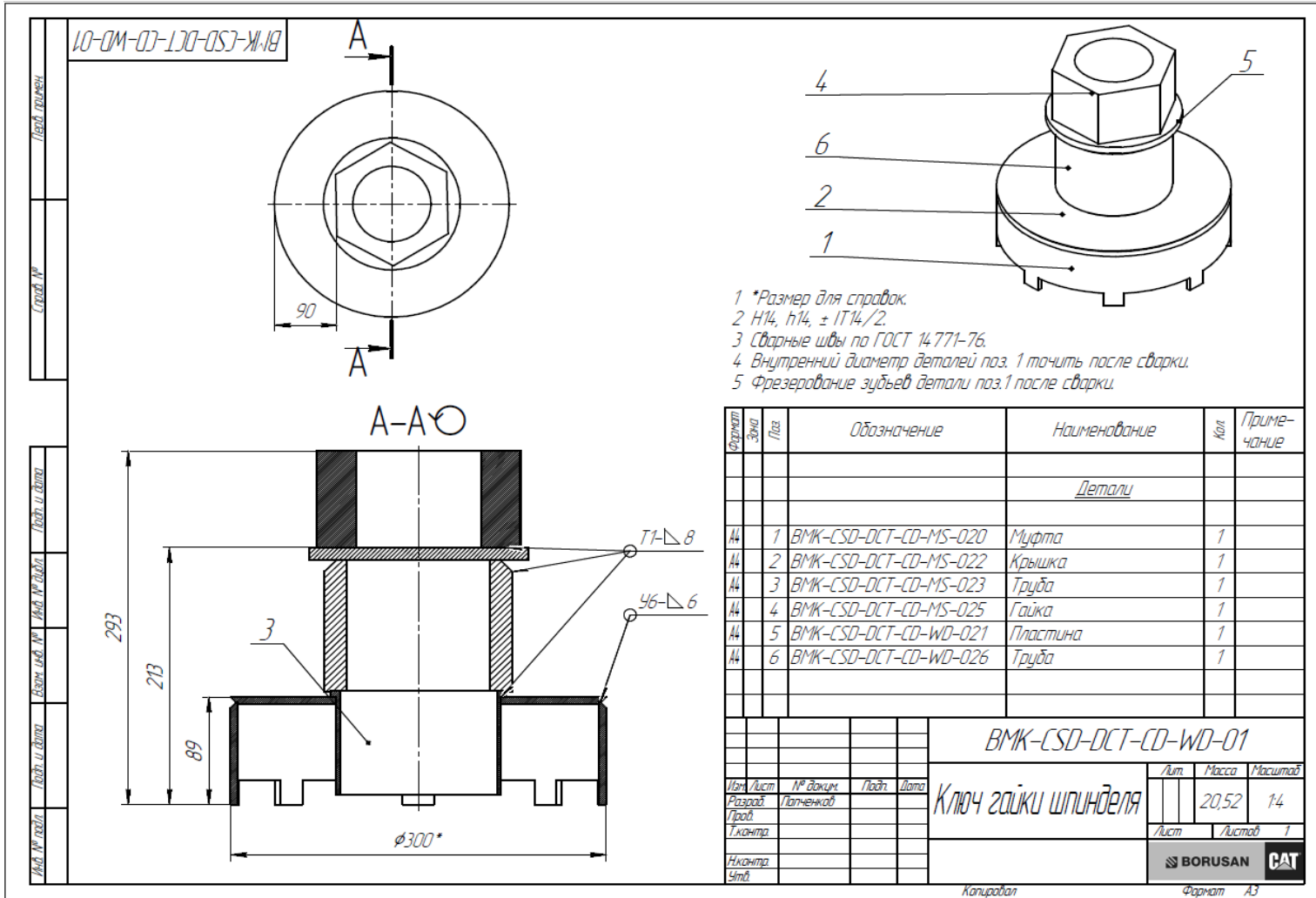
Drawing 1 wrench
